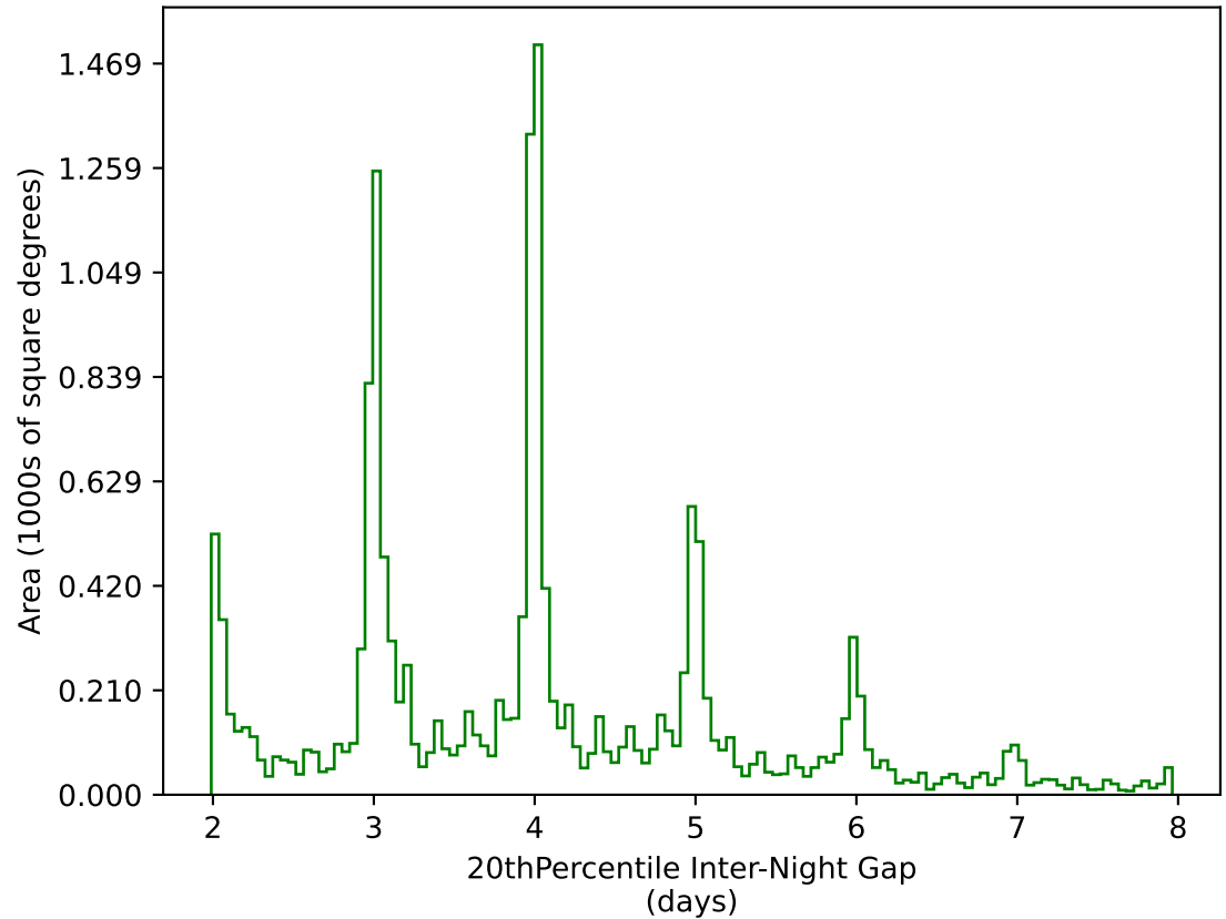
too_elab_r64_d2_griz_v3.4_10yrs WFD g band: 20thPercentile Inter-Night Gap
