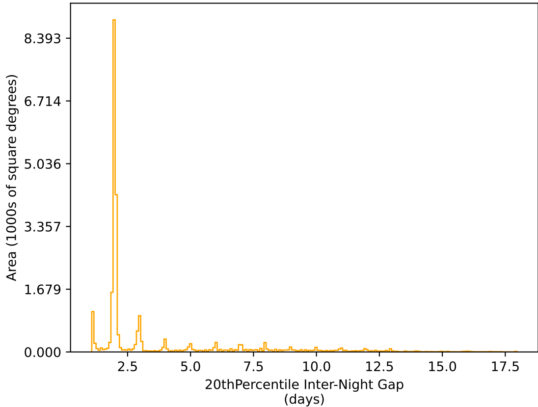
too_elab_r64_d2_griz_v3.4_10yrs All sky r band: 20thPercentile Inter-Night Gap
