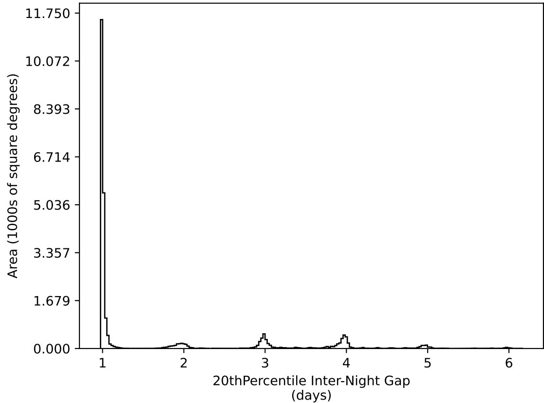
too_elab_r64_d2_griz_v3.4_10yrs All sky all bands: 20thPercentile Inter-Night Gap
