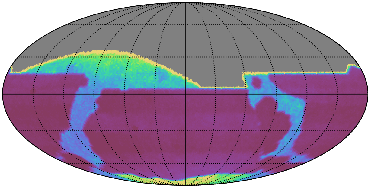
too_elab_r64_d2_griz_v3.4_10yrs : properMotion
