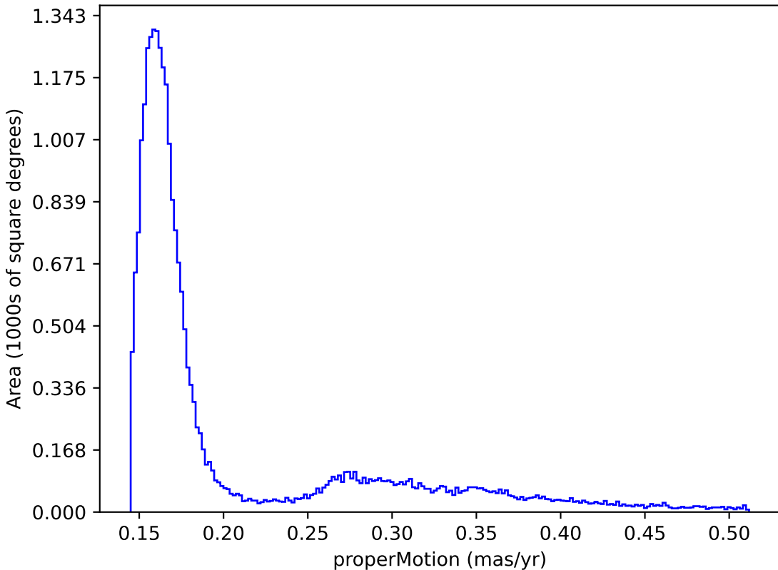
too_elab_r64_d2_griz_v3.4_10yrs : properMotion
