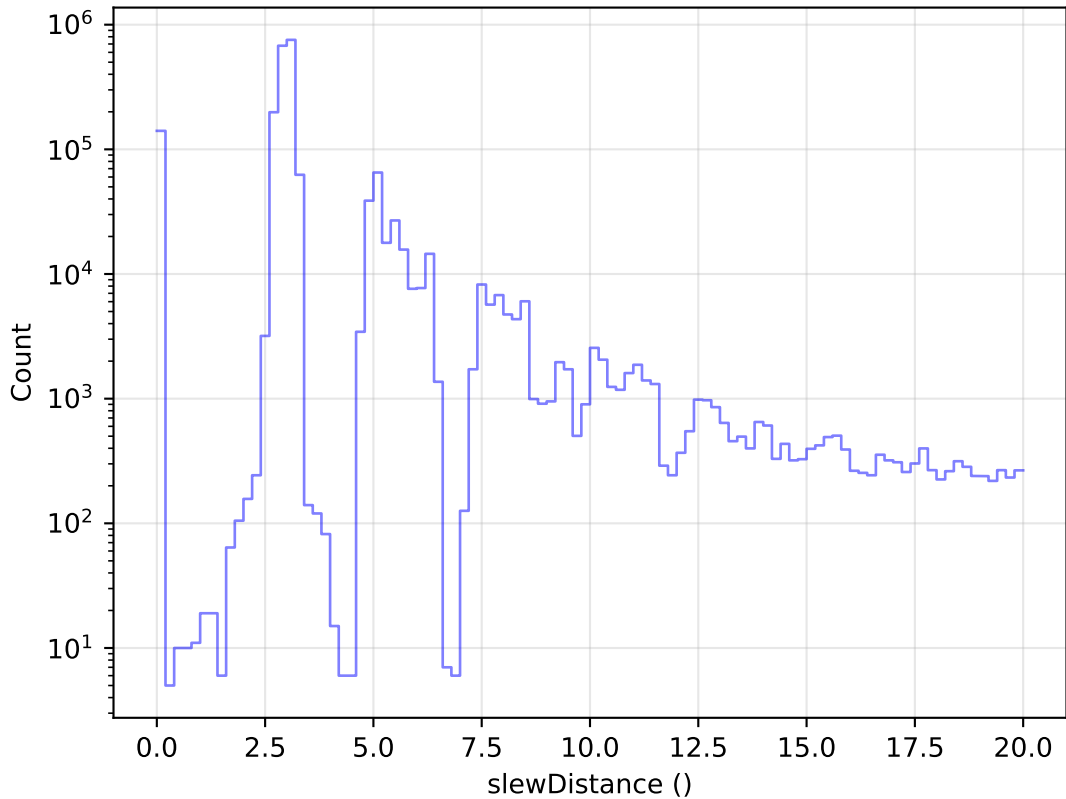
too_elab_r64_d2_griz_v3.4_10yrs All visits: Zoom Slew Distance Histogram
