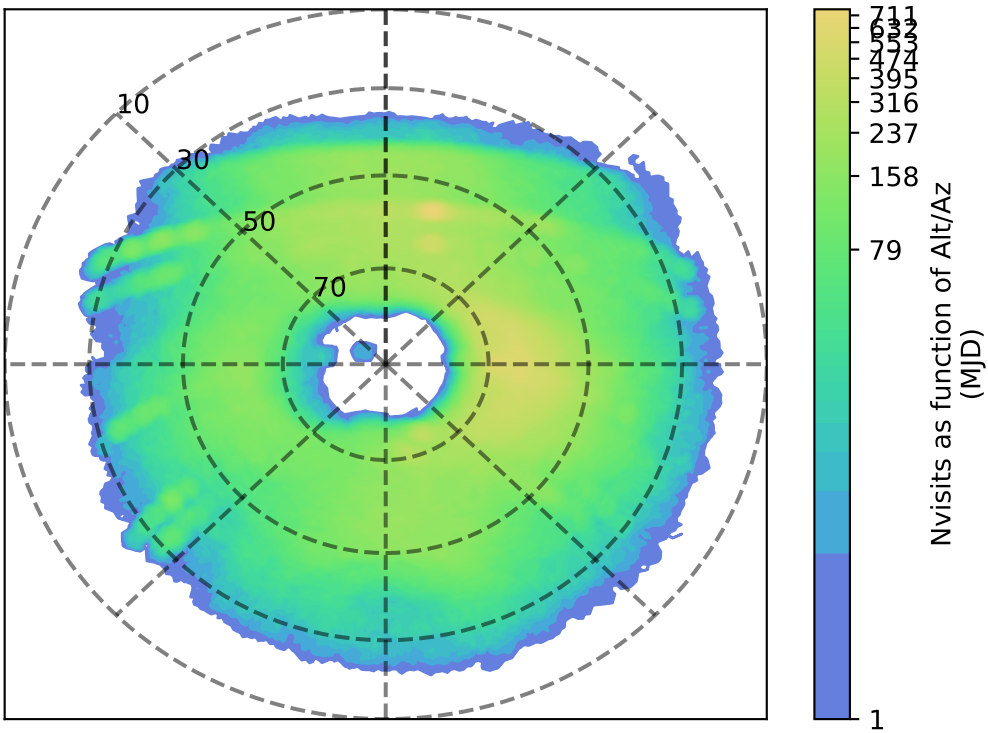
too_elab_r64_d2_griz_v3.4_10yrs u: Nvisits as function of Alt/Az
