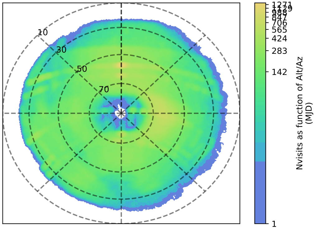
too_elab_r64_d2_griz_v3.4_10yrs g: Nvisits as function of Alt/Az
