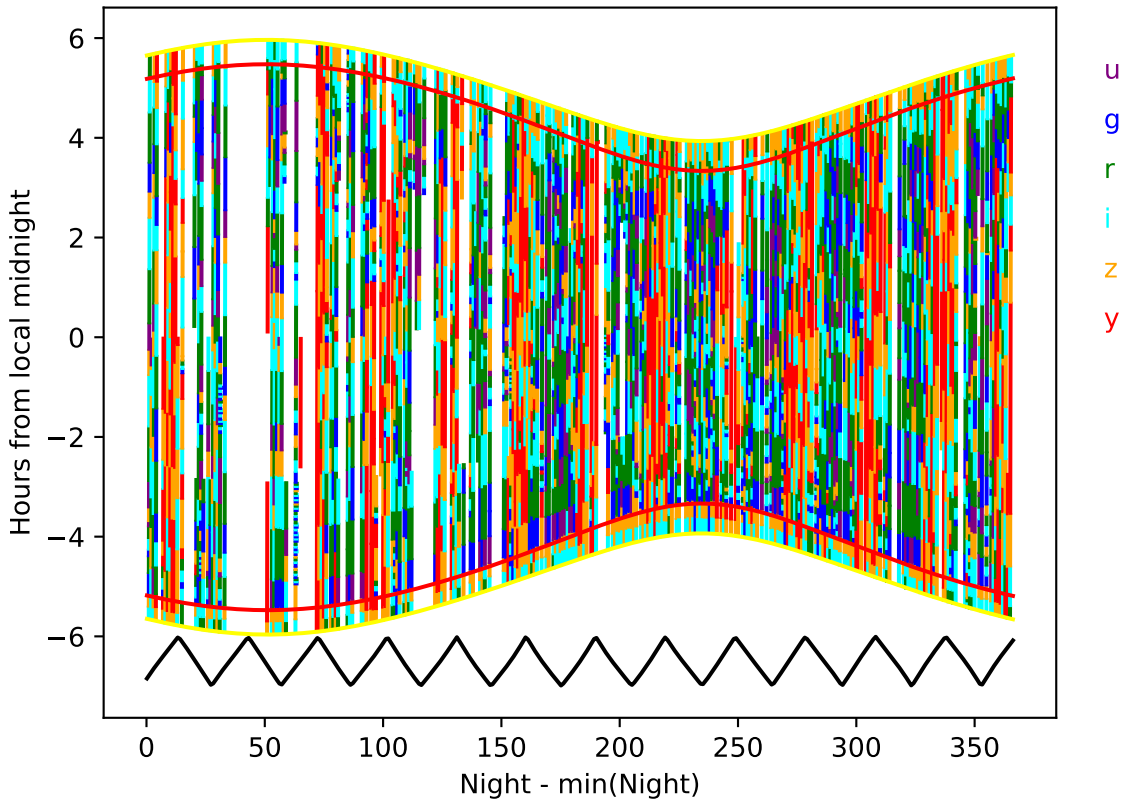
too_elab_r64_d2_griz_v3.4_10yrs year 8-9: Hourglass
