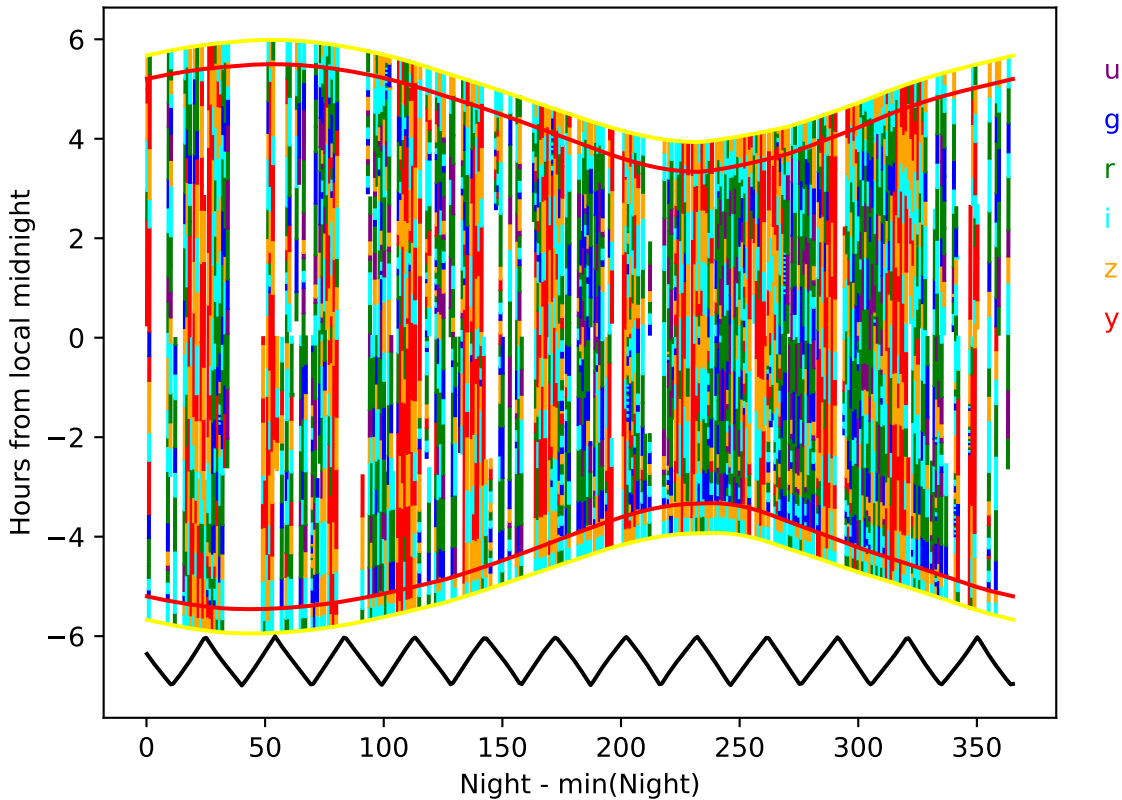
too_elab_r64_d2_griz_v3.4_10yrs year 4-5: Hourglass
