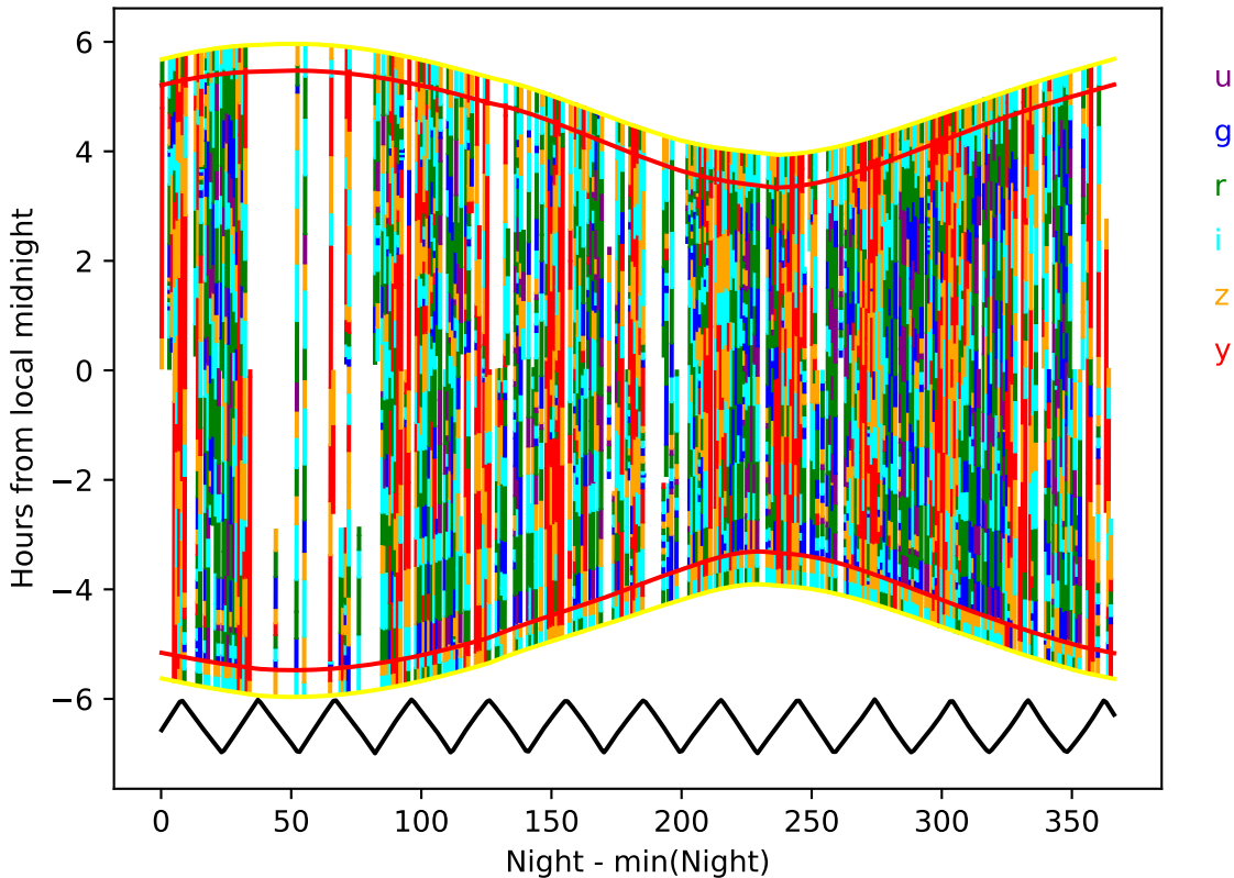
too_elab_r64_d2_griz_v3.4_10yrs year 3-4: Hourglass
