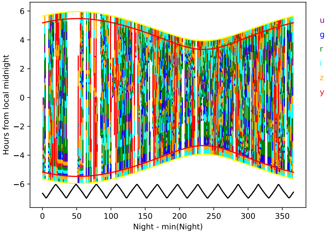
too_elab_r64_d2_griz_v3.4_10yrs year 2-3: Hourglass
