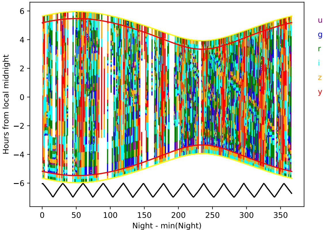
too_elab_r64_d2_griz_v3.4_10yrs year 1-2: Hourglass
