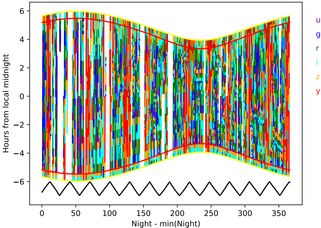
too_elab_r64_d2_griz_v3.4_10yrs year 0-1: Hourglass
