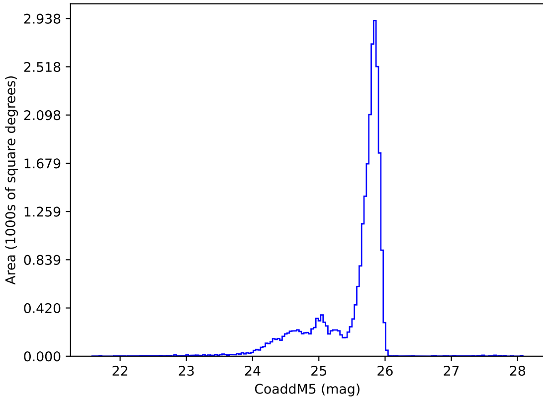
too_elab_r64_d2_griz_v3.4_10yrs z: CoaddM5
