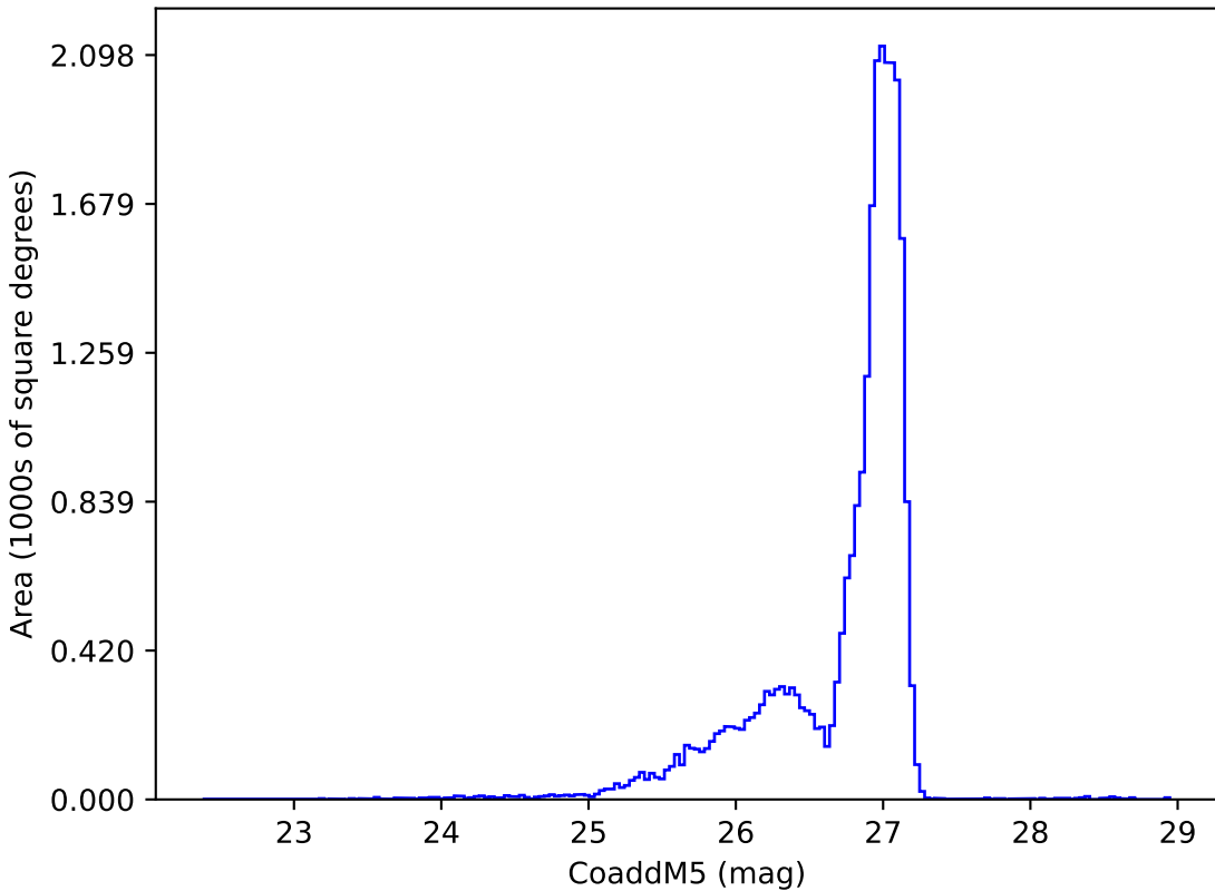
too_elab_r64_d2_griz_v3.4_10yrs r: CoaddM5
