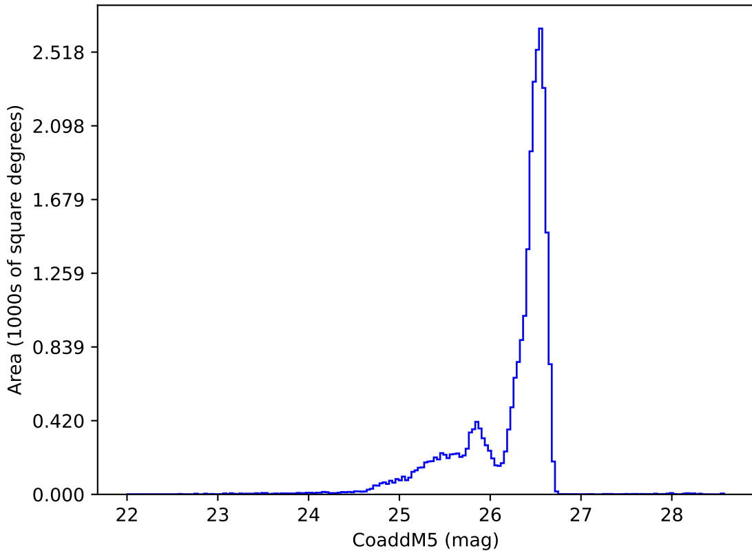
too_elab_r64_d2_griz_v3.4_10yrs i: CoaddM5
