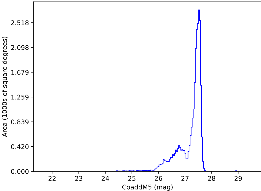
too_elab_r64_d2_griz_v3.4_10yrs : CoaddM5
