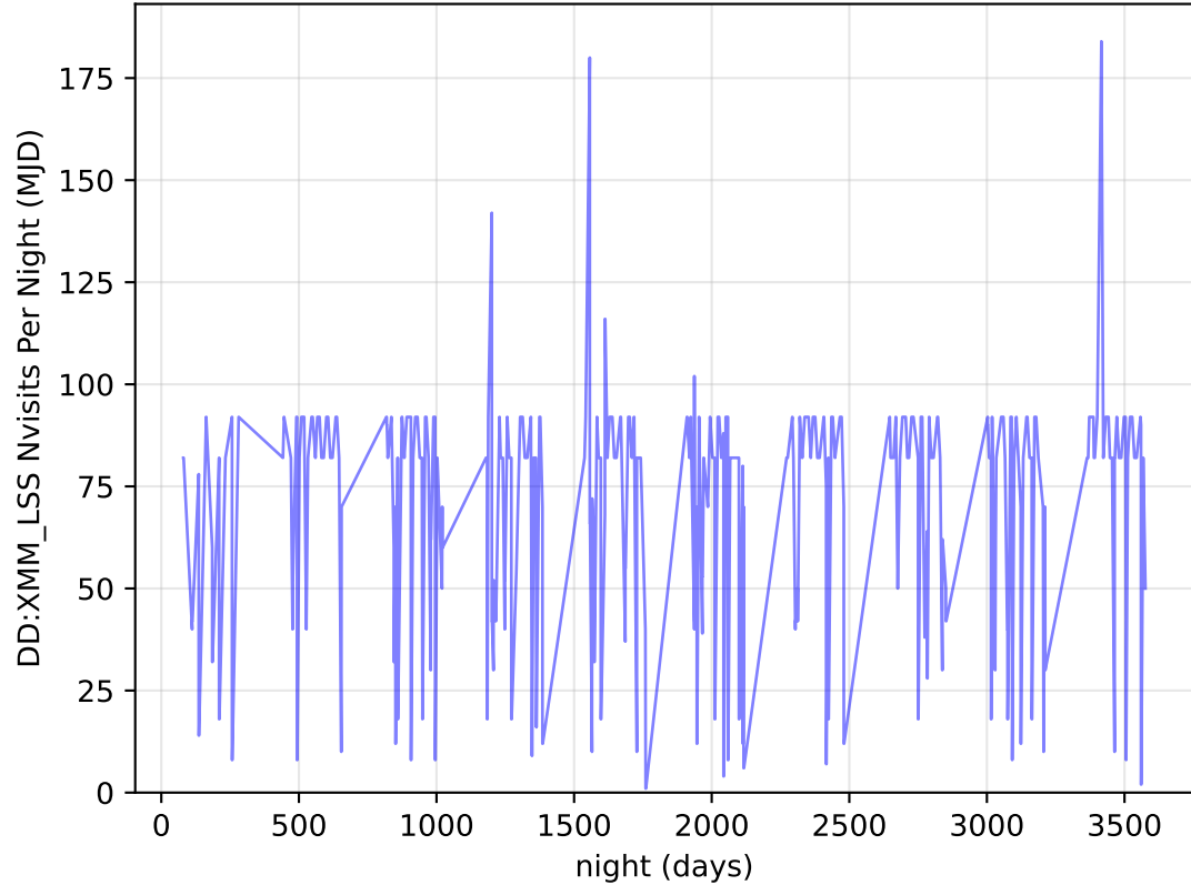
too_elab_r64_d2_griz_v3.4_10yrs all bands: DD:XMM_LSS Nvisits Per Night
