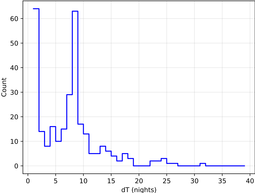
too_elab_r64_d2_griz_v3.4_10yrs all bands: DD:XMM_LSS Delta Nights Histogram
