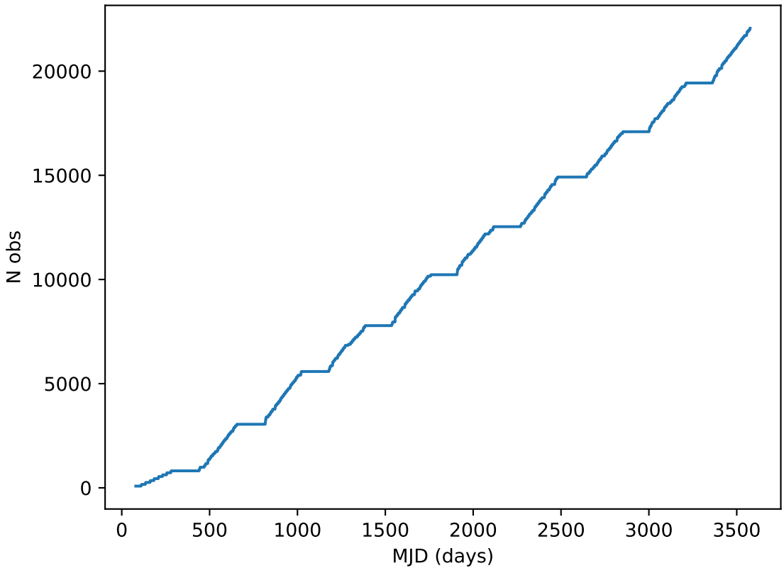
too_elab_r64_d2_griz_v3.4_10yrs all bands: DD:XMM_LSS Cumulative NVisits
