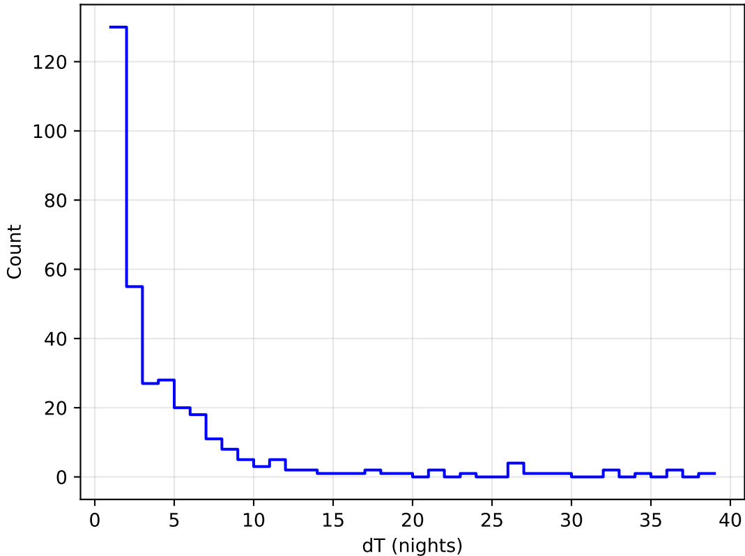
too_elab_r64_d2_griz_v3.4_10yrs all bands: DD:WFD Delta Nights Histogram
