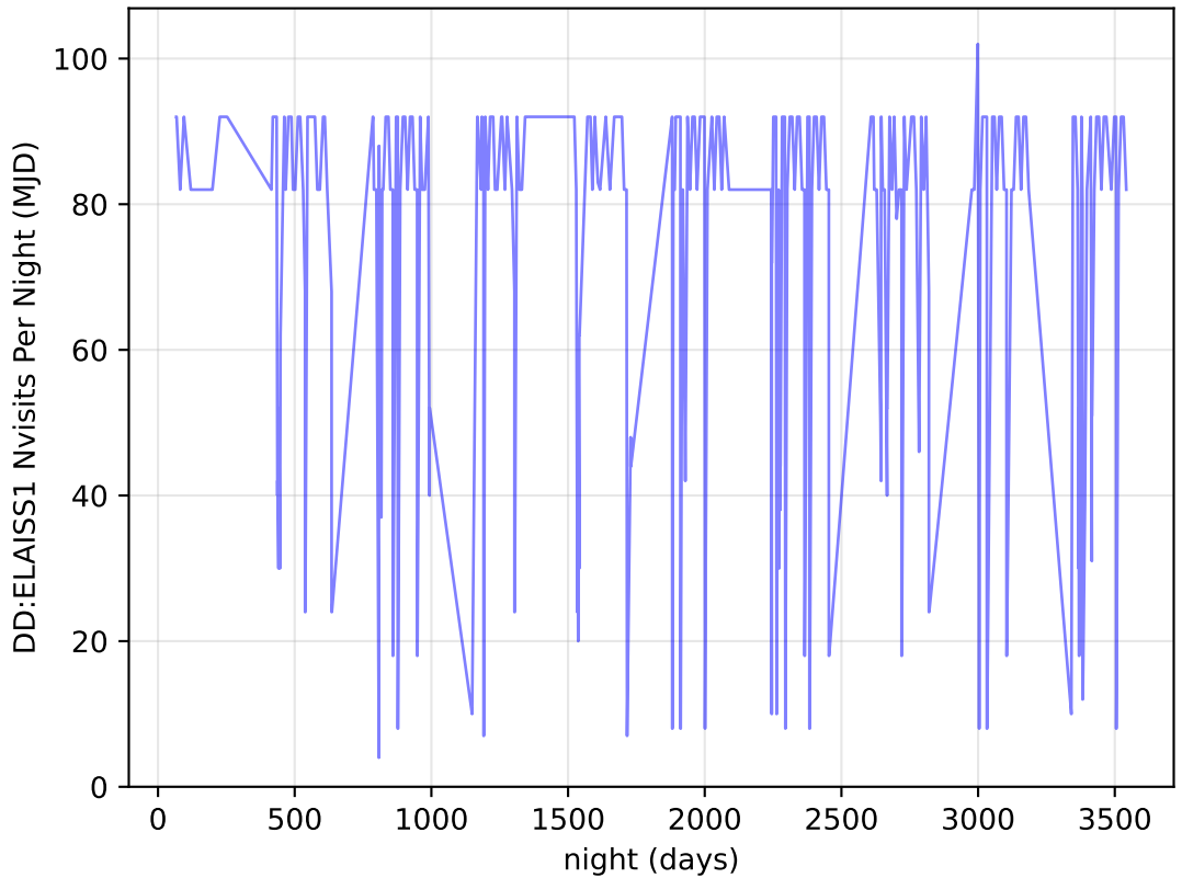
too_elab_r64_d2_griz_v3.4_10yrs all bands: DD:ELAISS1 Nvisits Per Night
