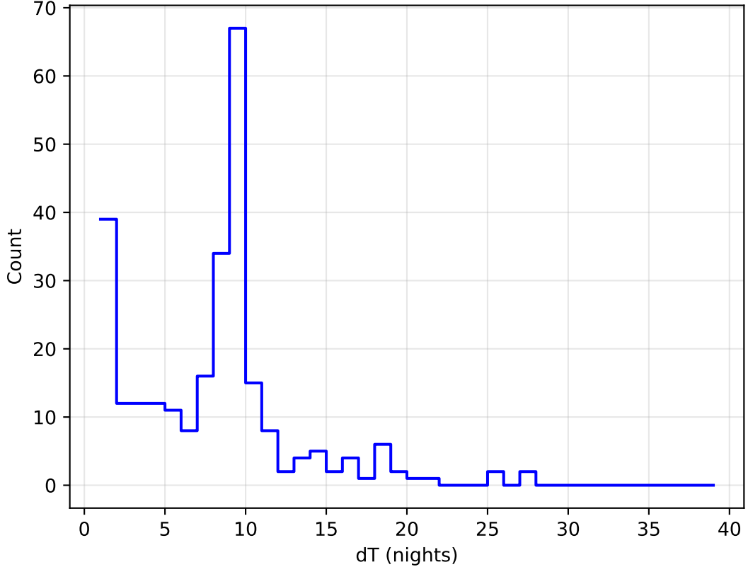
too_elab_r64_d2_griz_v3.4_10yrs all bands: DD:ELAISS1 Delta Nights Histogram
