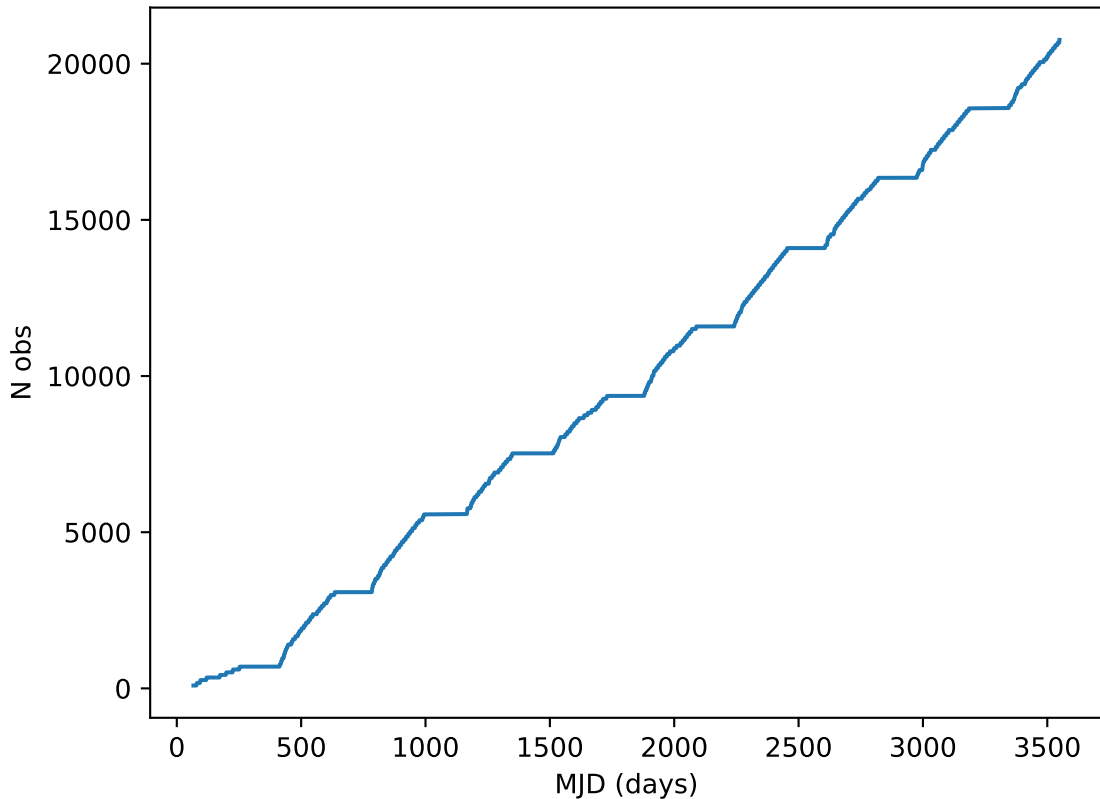
too_elab_r64_d2_griz_v3.4_10yrs all bands: DD:ELAISS1 Cumulative NVisits
