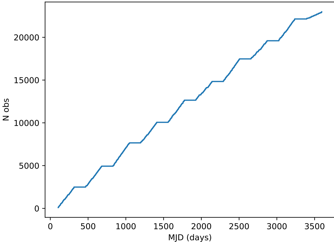
too_elab_r64_d2_griz_v3.4_10yrs all bands: DD:EDFS Cumulative NVisits
