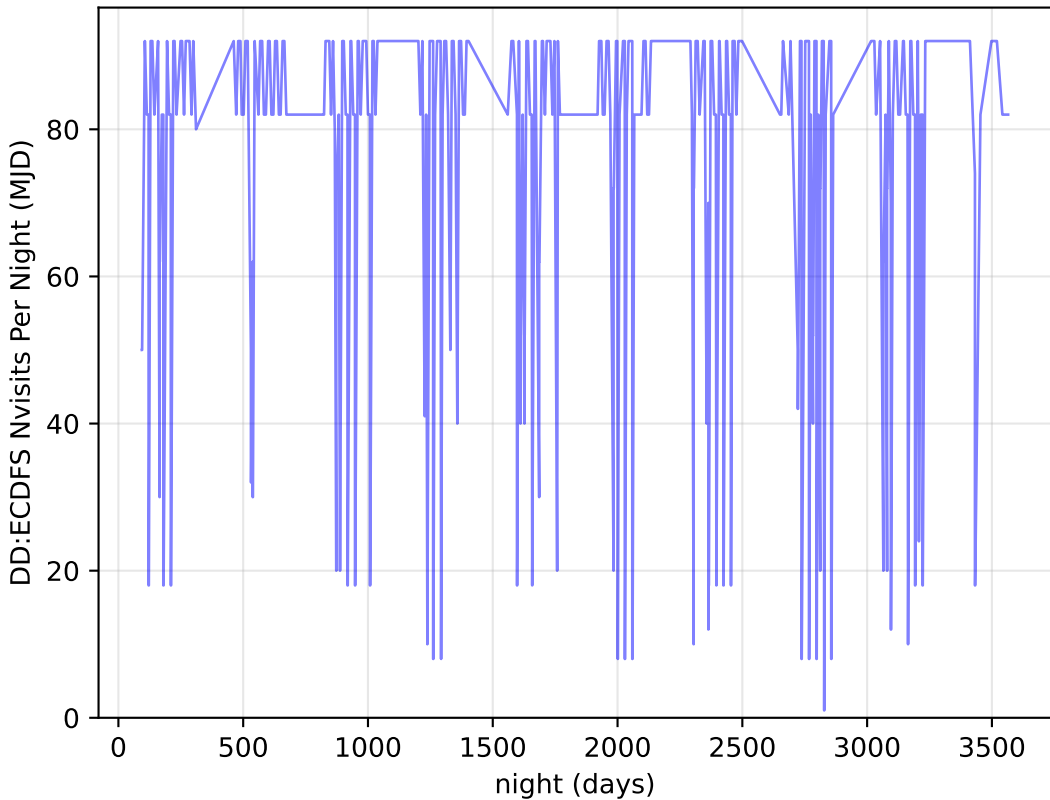
too_elab_r64_d2_griz_v3.4_10yrs all bands: DD:ECDFS Nvisits Per Night
