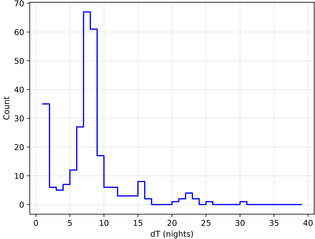
too_elab_r64_d2_griz_v3.4_10yrs all bands: DD:ECDFS Delta Nights Histogram
