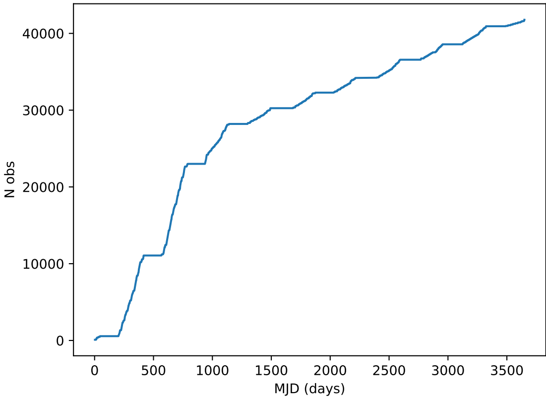
too_elab_r64_d2_griz_v3.4_10yrs all bands: DD: COSMOS Cumulative NVisits
