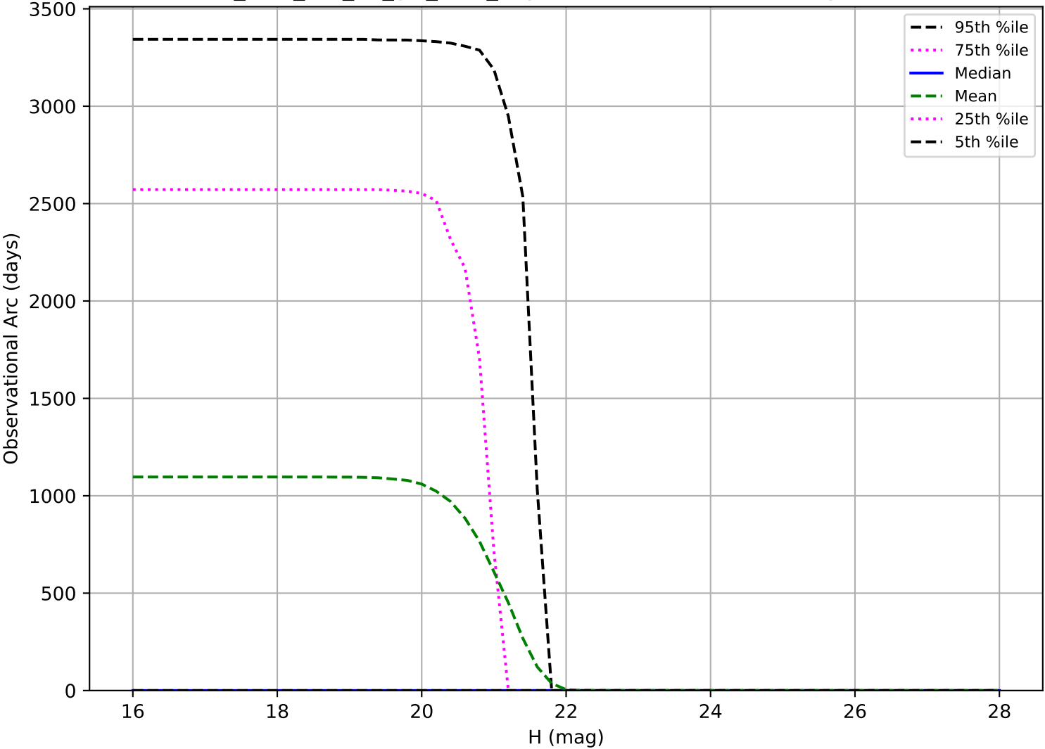
too_elab_r64_d2_giz_v3.4_10yrs: Observational Arc Length Vatira
