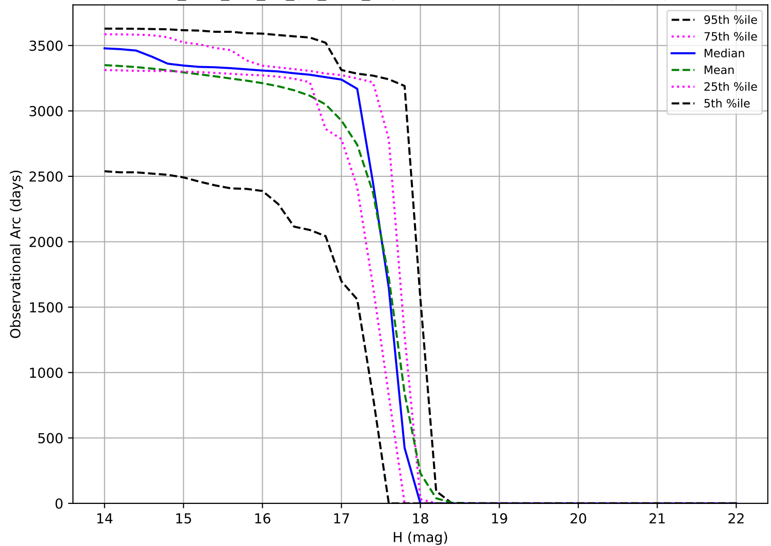
too_elab_r64_d2_giz_v3.4_10yrs: Observational Arc Length Trojan
