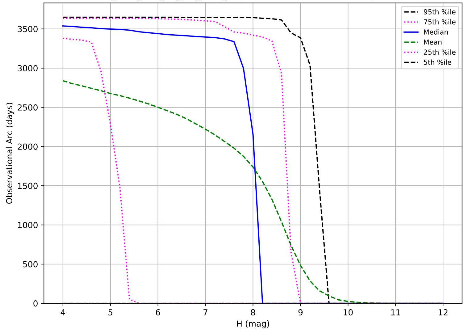
too_elab_r64_d2_giz_v3.4_10yrs: Observational Arc Length TNO
