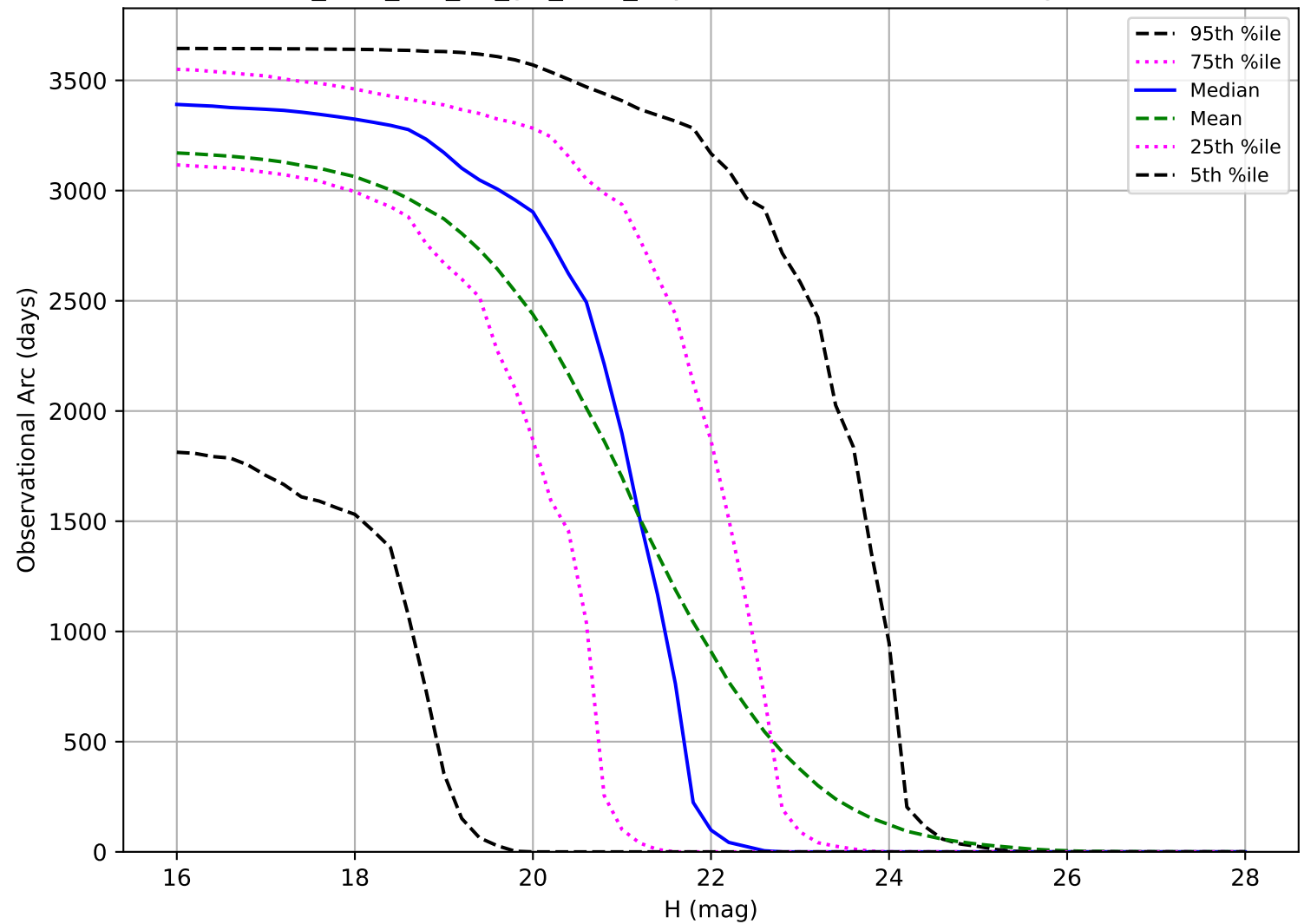
too_elab_r64_d2_giz_v3.4_10yrs: Observational Arc Length NEO
