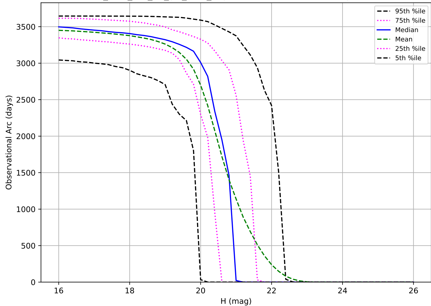
too_elab_r64_d2_giz_v3.4_10yrs: Observational Arc Length MBA
