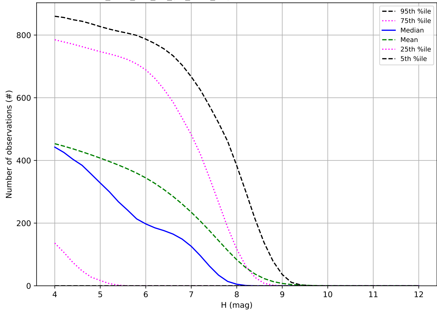
too_elab_r64_d2_giz_v3.4_10yrs: Number of observations TNO
