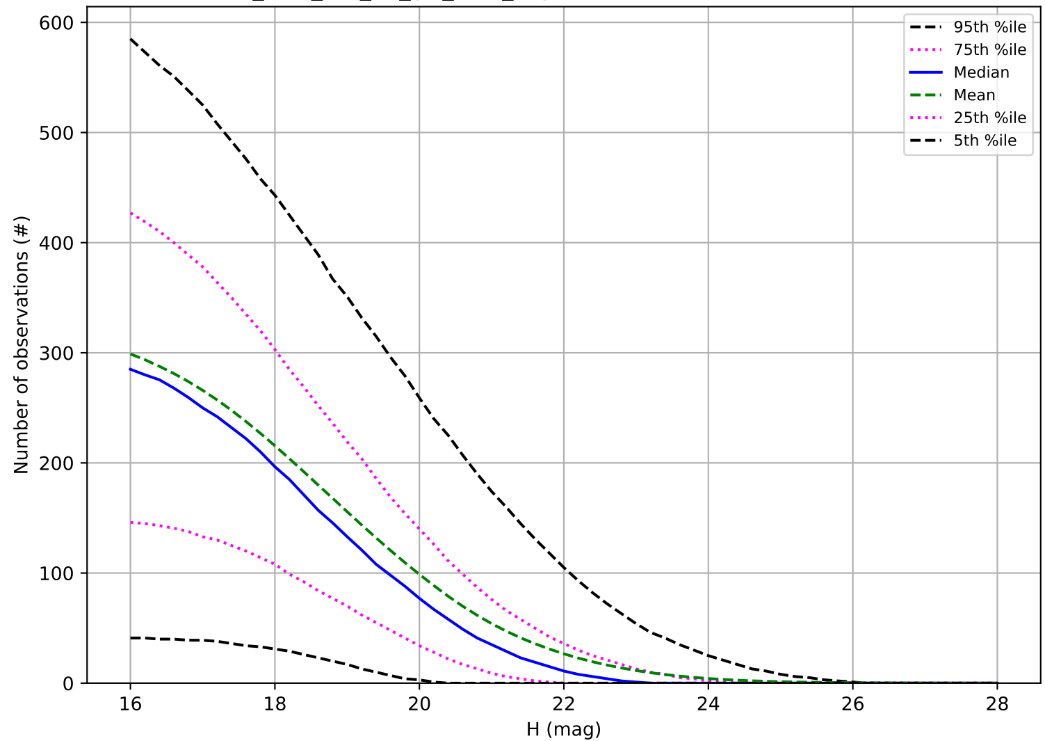
too_elab_r64_d2_giz_v3.4_10yrs: Number of observations PHA
