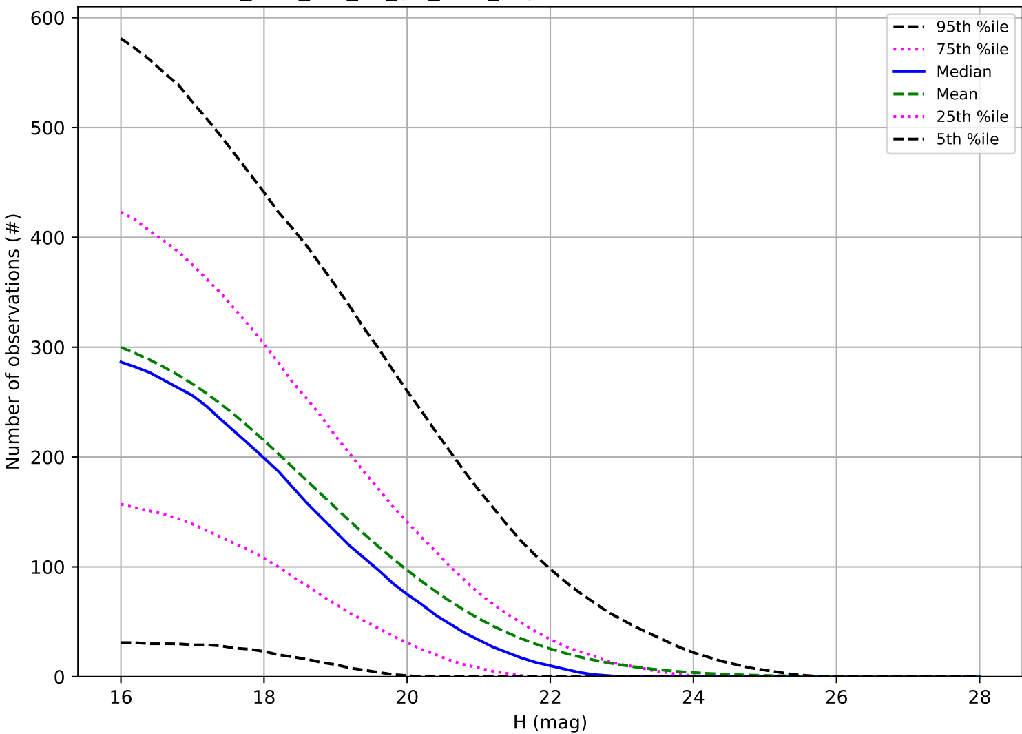
too_elab_r64_d2_giz_v3.4_10yrs: Number of observations NEO
