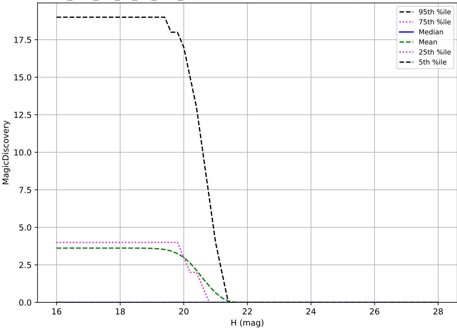
too_elab_r64_d2_giz_v3.4_10yrs: Vatira 6 detections in 60 nights detection loss
