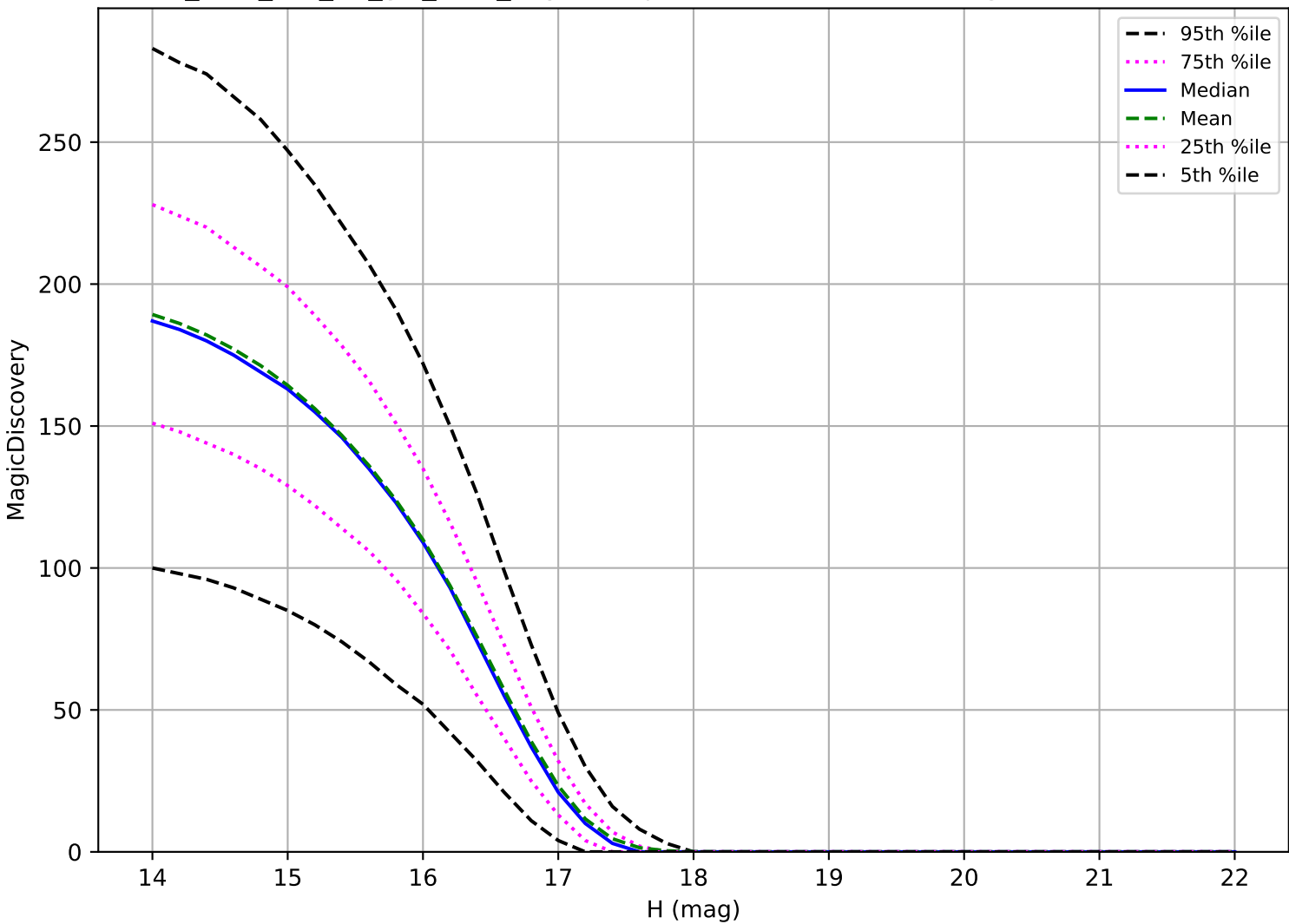
too_elab_r64_d2_giz_v3.4_10yrs: Trojan 6 detections in 60 nights detection loss
