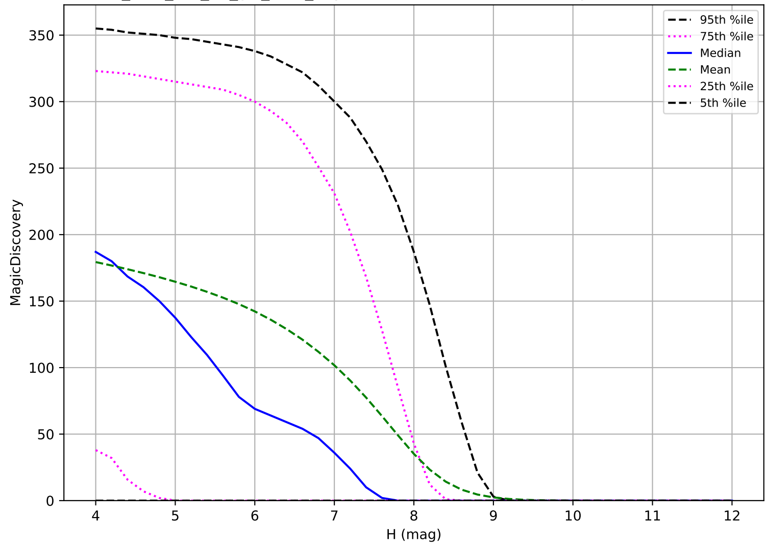
too_elab_r64_d2_giz_v3.4_10yrs: TNO 6 detections in 60 nights detection loss
