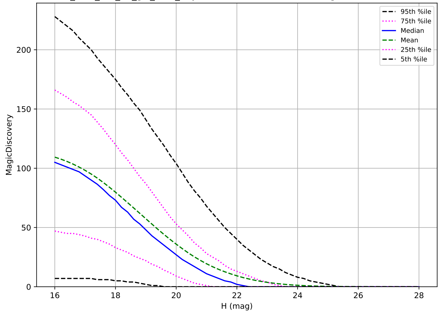
too_elab_r64_d2_giz_v3.4_10yrs: PHA 6 detections in 60 nights detection loss
