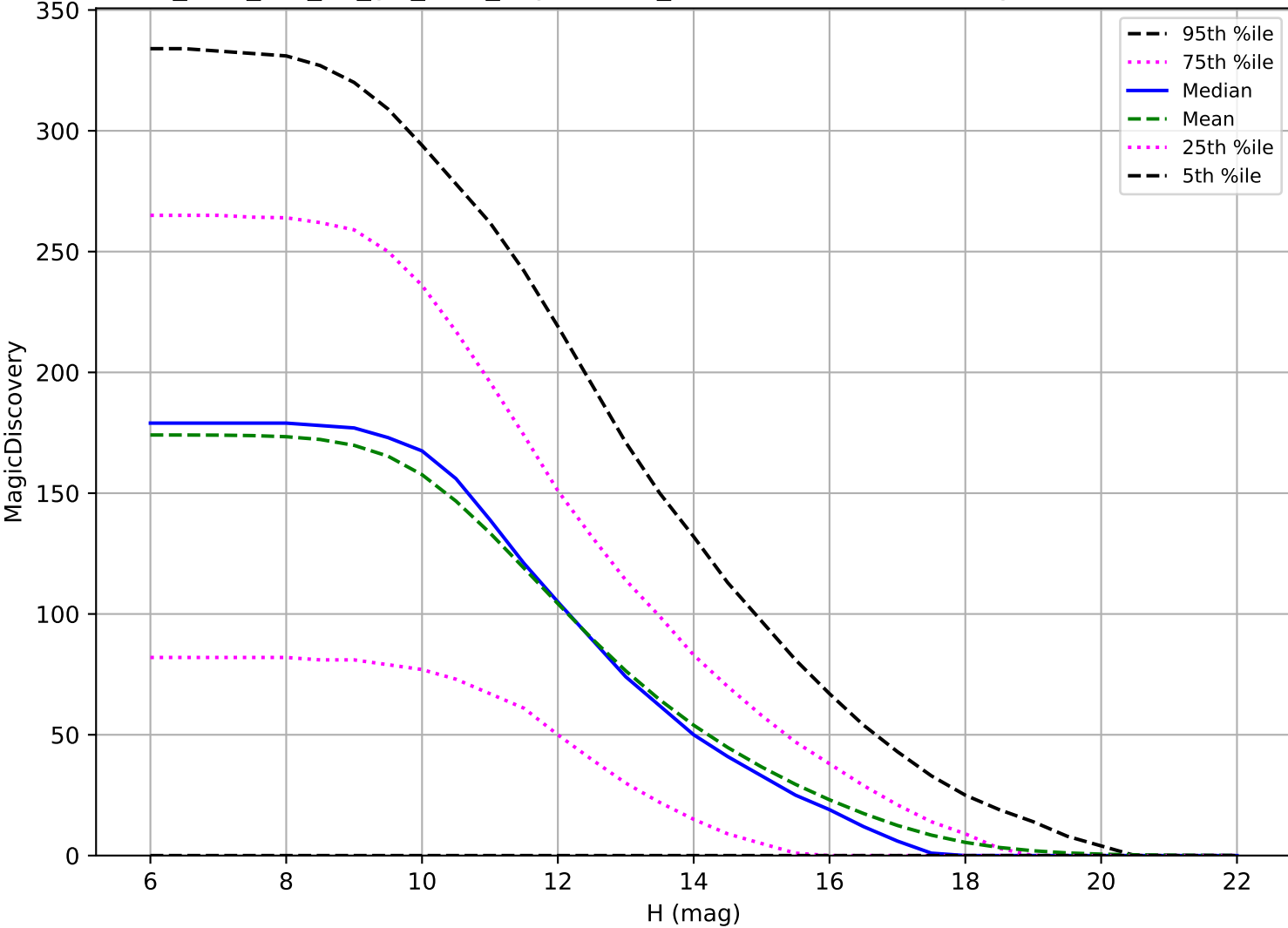
too_elab_r64_d2_giz_v3.4_10yrs: OCC_r5 6 detections in 60 nights detection loss
