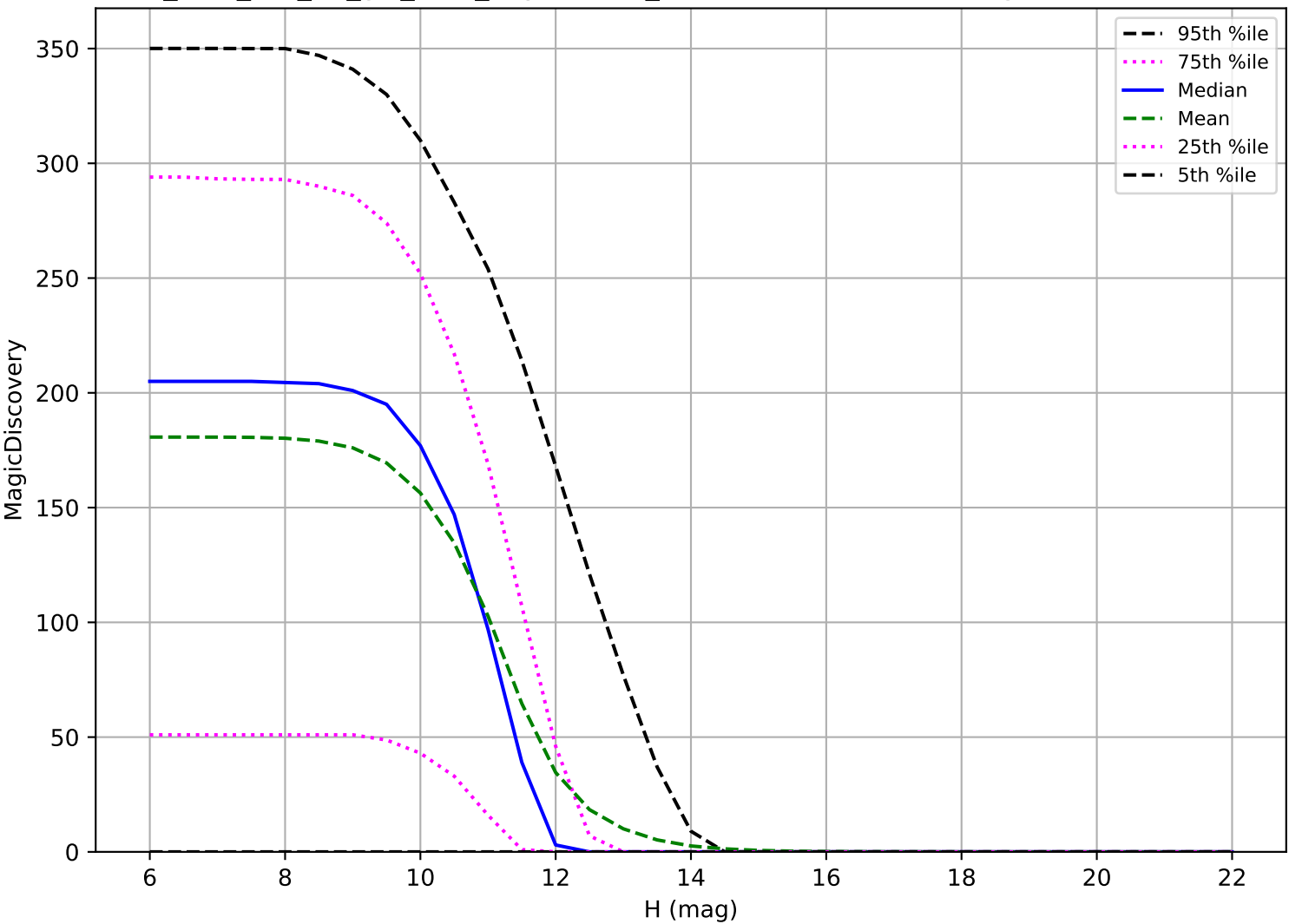
too_elab_r64_d2_giz_v3.4_10yrs: OCC_r20 6 detections in 60 nights detection loss
