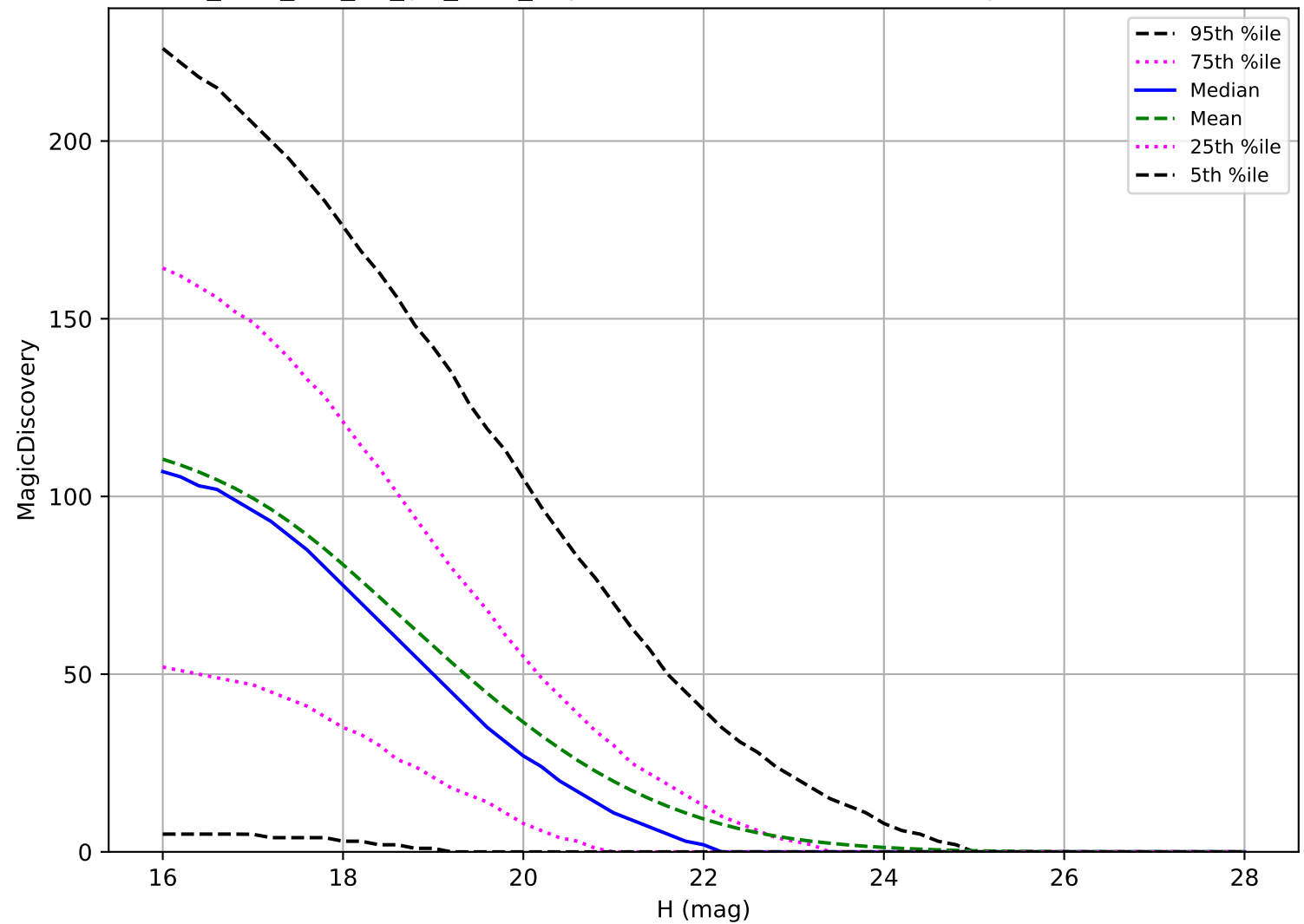
too_elab_r64_d2_giz_v3.4_10yrs: NEO 6 detections in 60 nights detection loss
