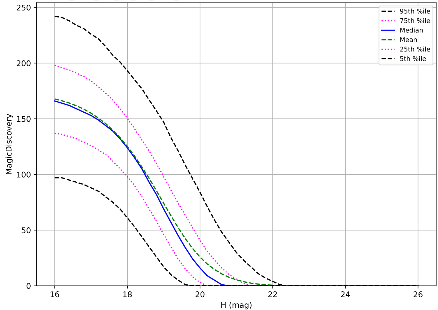
too_elab_r64_d2_giz_v3.4_10yrs: MBA 6 detections in 60 nights detection loss
