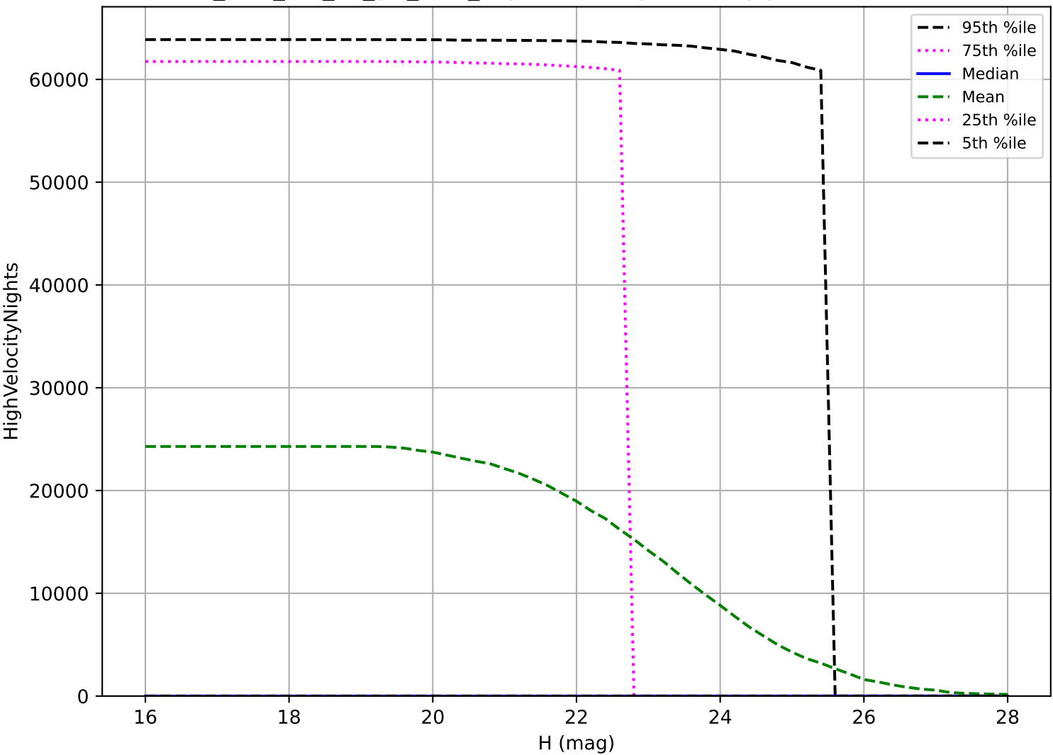
too_elab_r64_d2_giz_v3.4_10yrs: PHA High velocity pair detection loss
