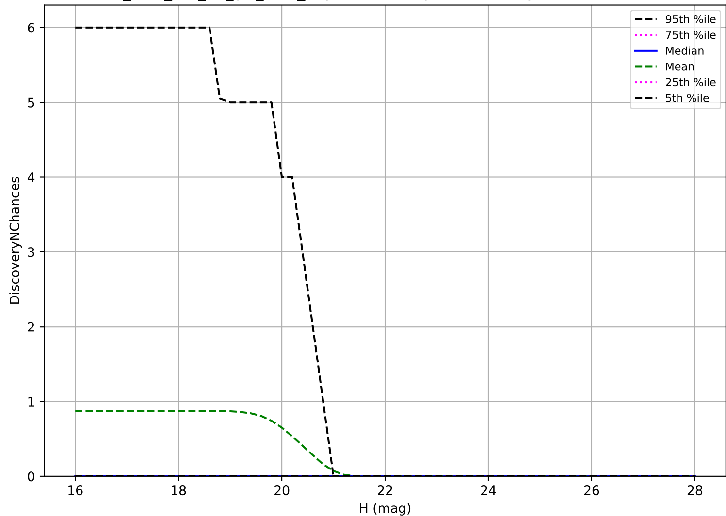
too_elab_r64_d2_giz_v3.4_10yrs: Vatira 3 pairs in 15 nights detection loss
