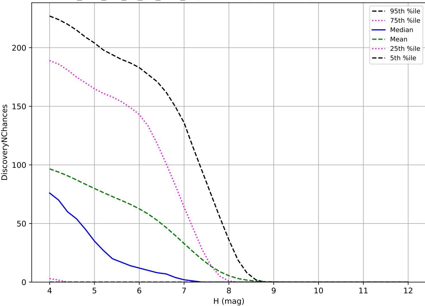
too_elab_r64_d2_giz_v3.4_10yrs: TNO 3 pairs in 15 nights detection loss
