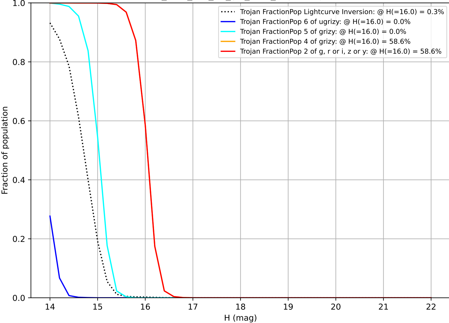
too_elab_r64_d2_giz_v3.4_10yrs Trojan
