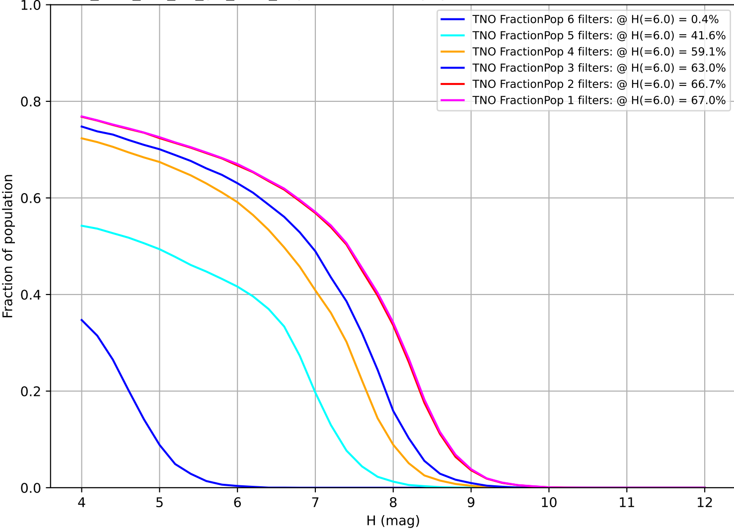
too_elab_r64_d2_giz_v3.4_10yrs: Fraction of population with colors in X filters TNO
